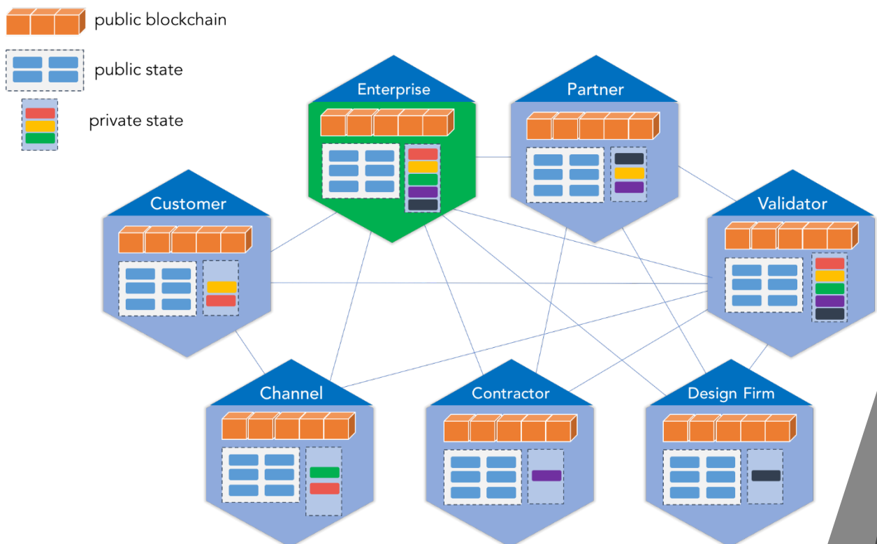
Figure 3: Blending Public & Private States
